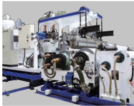
Extruder with Automatic T-Die & Casting Unit
